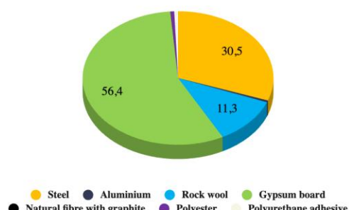
Material composition of swing gate
